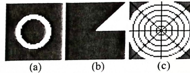
Fig. 1. (a) Ring filter, (b) Wedge filter of 45° (c) Tessels obtained with the product of rings and wedge filters
